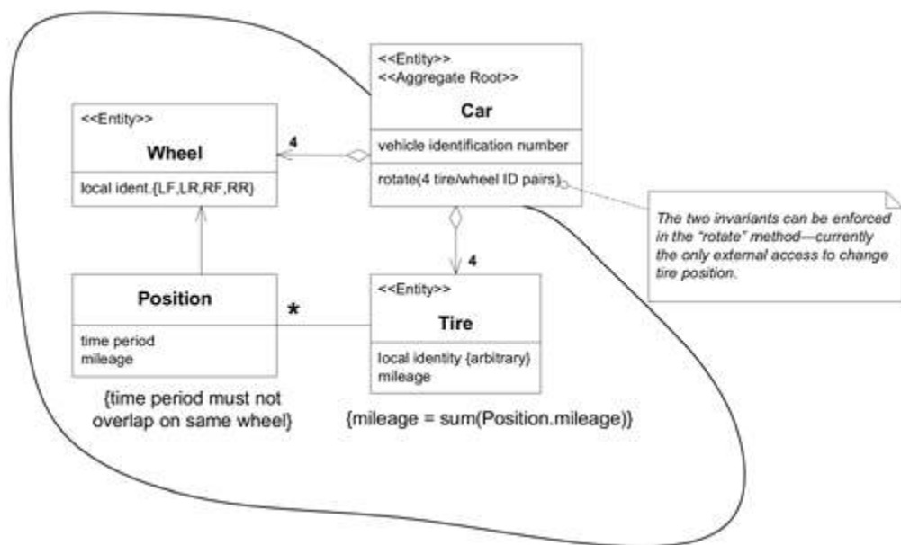
Figure 6.3. AGGREGATE invariants
